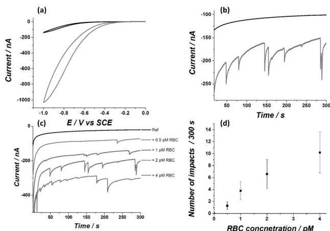
Figure 3. a) Voltammetry of a solution containing 20 mM \text{H}_2\text{O}_2 (black) and with 2 pM RBC (gray) on a carbon wire. Voltammograms were performed under a 50 \text{ mV s}^{-1} scan rate. b) Chronoamperograms of a 20 mM hydrogen peroxide solution (black curve) and with 2 pM RBC (gray curve) under an applied potential of -0.8 \text{ V} versus SCE. c) Chronoamperograms of 20 mM hydrogen peroxide with various concentrations of RBC in solution under an applied potential of -0.8 \text{ V} versus SCE. The y axis was offset for clarity. d) Average spike frequencies during a 300 second scan as a function of RBC concentration.
