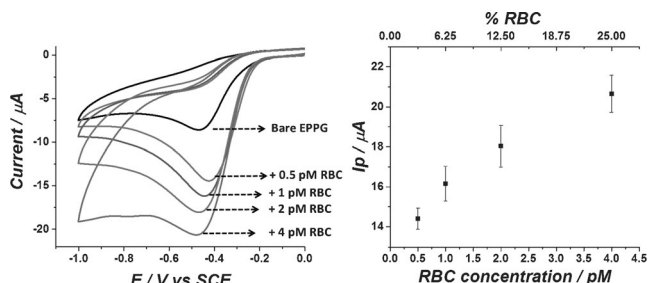
Figure 1. a) Voltammetry of a 5 \mu\text{L} RBC drop-cast on an EPPG electrode, from solutions with designated initial concentration. b) The peak current (absolute values) as a function of initial RBC concentration drop cast. For all measurements a 50 \text{ mVs}^{-1} scan rate was used.
